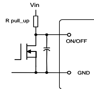
Fig. 13. Circuit for Negative Logic Control
