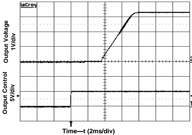
Figure 5. Start-Up from Enable Control Input voltage 5V, Output current 20A
