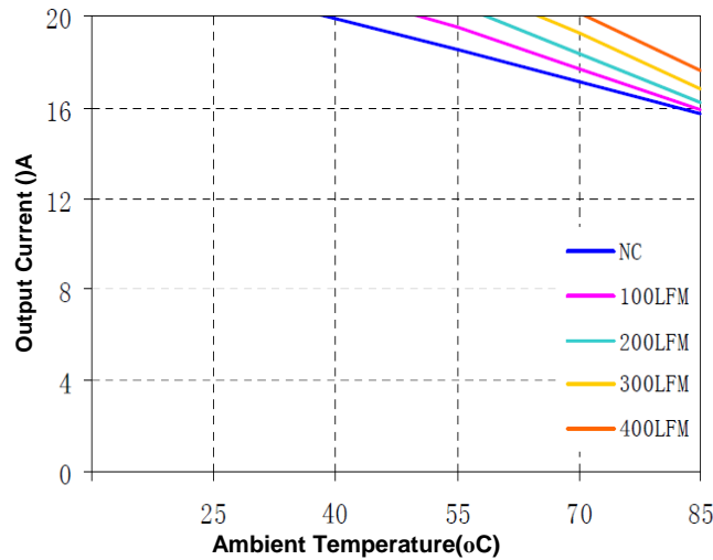
Figure 11(c) Current Derating Curve for 1.5V Output (Vin = 5V open frame)
