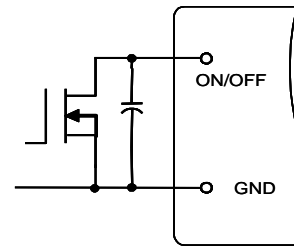
Fig. 12. Circuit for Positive Logic Control
