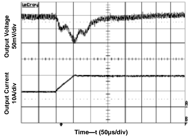
Figure 8 Transient Load Response Input voltage 5V, Output current 6A(50% full load), Slew rate 0.2A/µs
