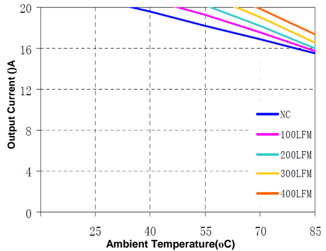
Figure 11(d) Current Derating Curve for 1.8V Output (Vin = 5V open frame)
