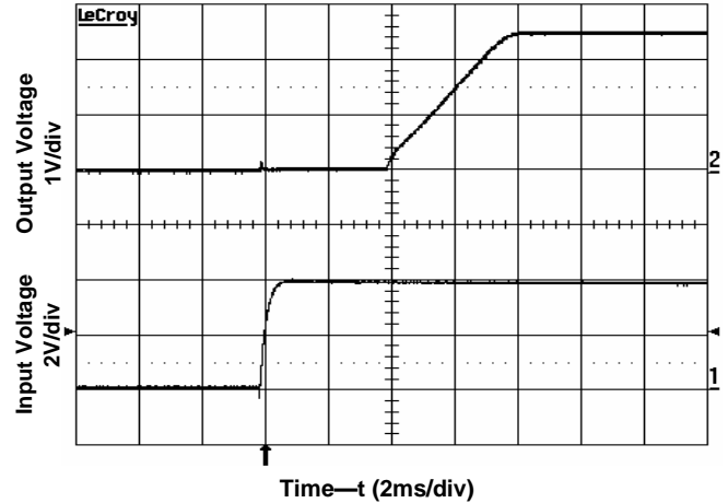
Figure 6. Start-up Application of Input Voltage Input voltage 4V, Output current 20A
