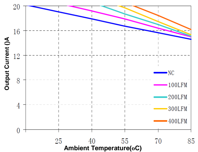
Figure 11(f) Current Derating Curve for 3.3V Output (Vin = 5V open frame)
