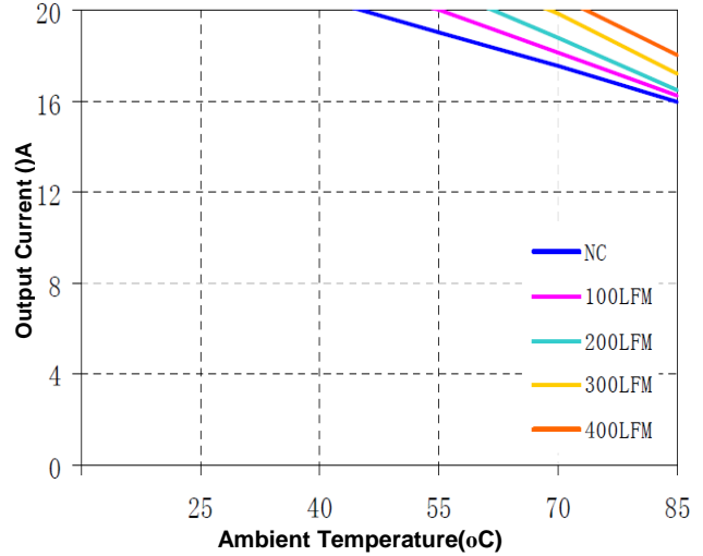
Figure 11(b) Current Derating Curve for 1.2V Output (Vin = 5V open frame)
