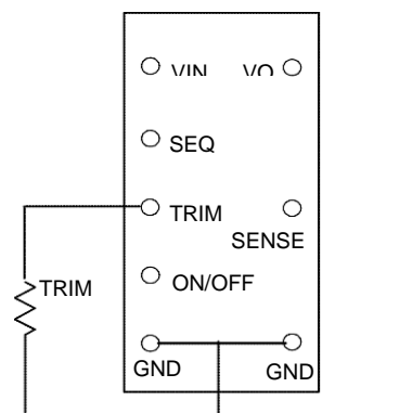
Fig. 14 Circuit to Trim Output Voltage.
