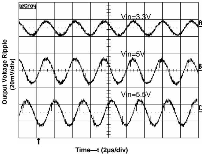
Figure 3. Output Ripple Voltage at 2.5V, 20A Output
