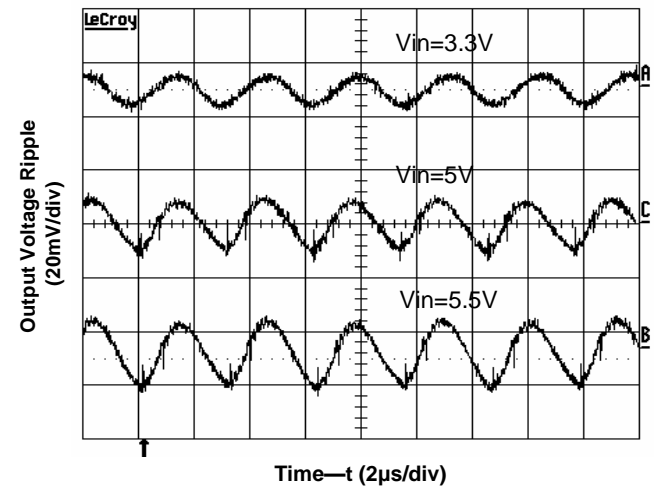
Figure 4. Output Ripple Voltage at 1V, 20A Output
