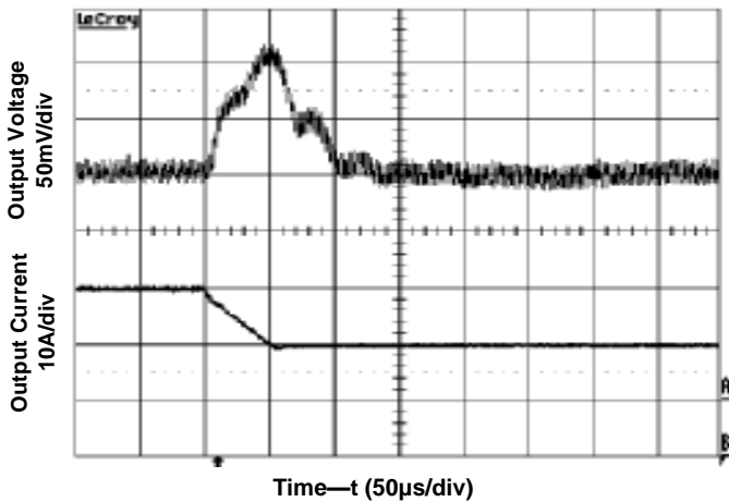
Figure 7 Transient Load Response Input voltage 5V, Output current 6A(50% full load), Slew rate 0.2A/µs.
