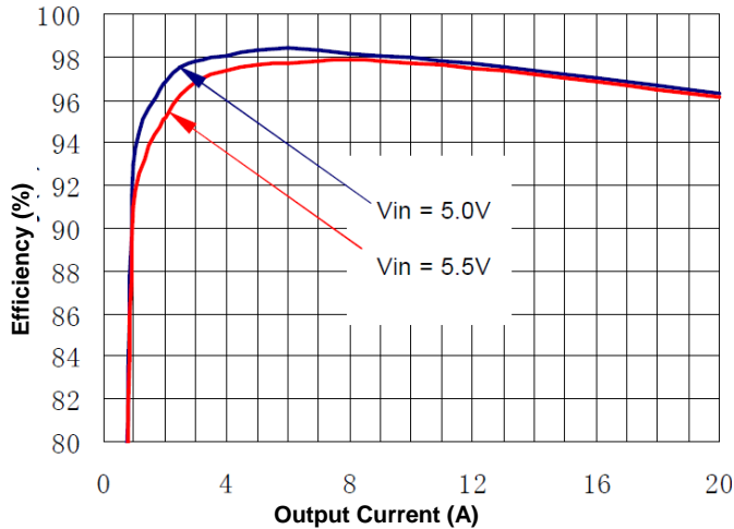
Figure 1(g). Efficiency vs. Load Current (25°C, 3.3V)
