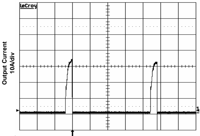
Figure 9. Short Circuit Current. Vin = 5V
