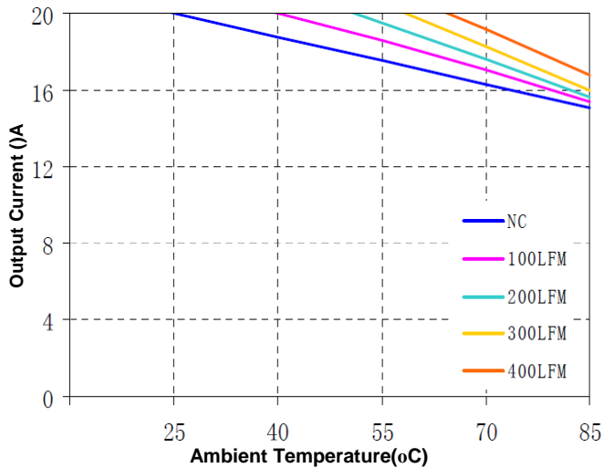
Figure 11(e) Current Derating Curve for 2.5V Output (Vin = 5V open frame)
