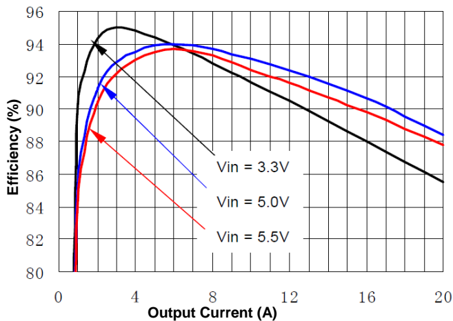
Figure 1(c). Efficiency vs. Load Current (25°C, 1.2V)
