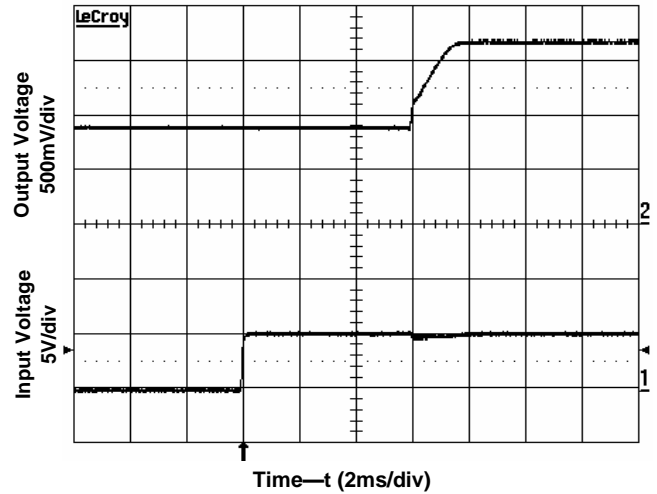
Figure 2. Start-Up with Prebias Input voltage 5V, Output current 0A, Output voltage 1.8V, Prebias 1.2V
