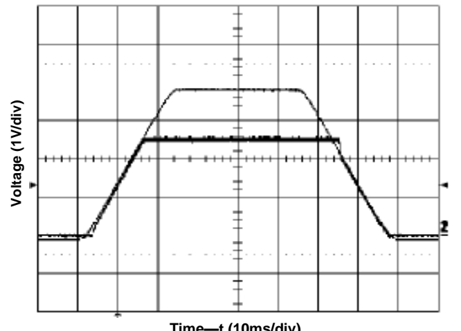
Figure 10. Voltage Tracking/Sequencing (with tracking option) Vin= 4V, Vo = 2.5V, Io = 0A
