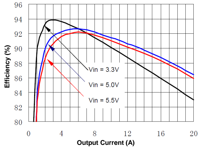
Figure 1(b). Efficiency vs. Load Current (25°C, 1.0V)
