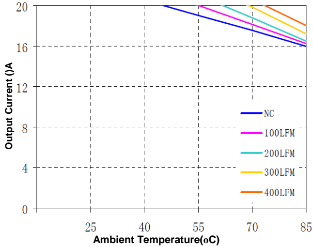
Figure 11(a) Current Derating Curve for 1.0V Output (Vin = 5V open frame)
