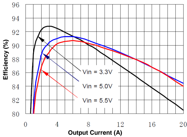
Figure 1(a). Efficiency vs. Load Current (25°C, 0.8V)
