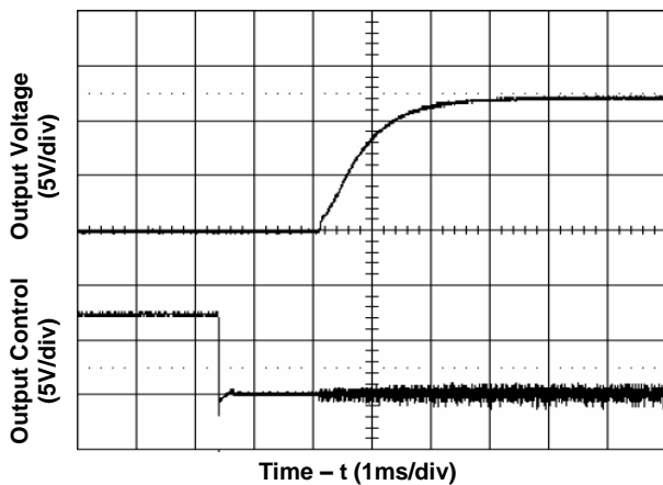
Figure 3. Start-Up from Enable Control Input voltage 36V, Output current 11A
