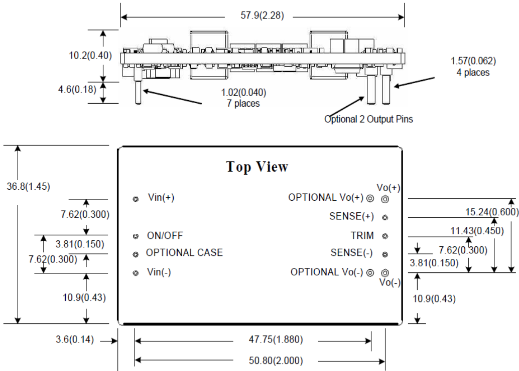
Figure 21. Open Frame Converter
