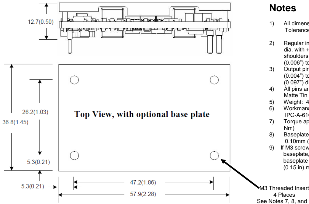
Figure 22. Converter with a baseplate
