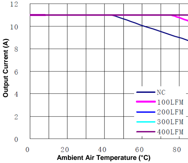
Figure 11. Current Derating Curve for Airflow Direction 3 (Ref. Fig. 12 for Airflow Direction; typical V_{in} , open frame unit using soldering interface)
