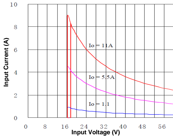
Figure 9. Input Characteristics
