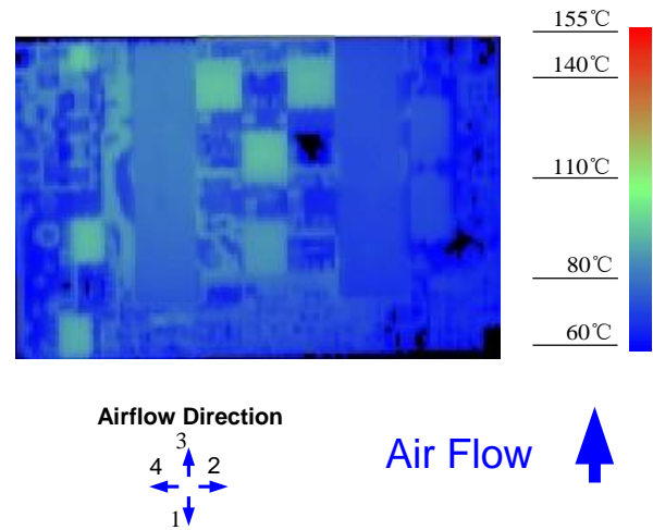
Figure 12. Thermal Image for Airflow Direction 3 (11A output, 55°C ambient, 200 LFM, typical V_{in} , open frame unit using soldering interface)
