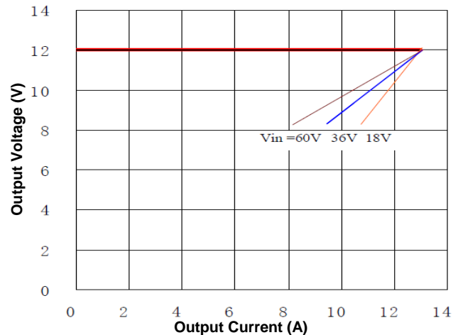
Figure 10. Output Characteristics
