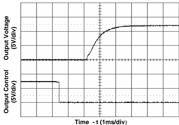
Figure 4. Start-Up from Enable Control Input voltage 36V, Output current 0A
