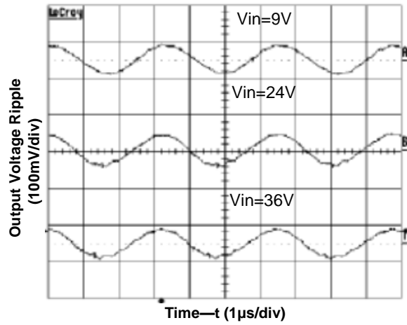
Figure 7. Output Reflected Ripple at 3.3V, 10A Output
