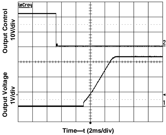
Figure 4. Start-Up from Enable Control Input voltage 24V, Output current 0A 3.3V.
