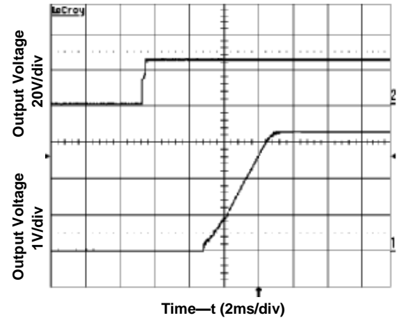
Figure 5. Start-Up from Application of Input Voltage (Input voltage 24V, Output current 10A 3.3V)
