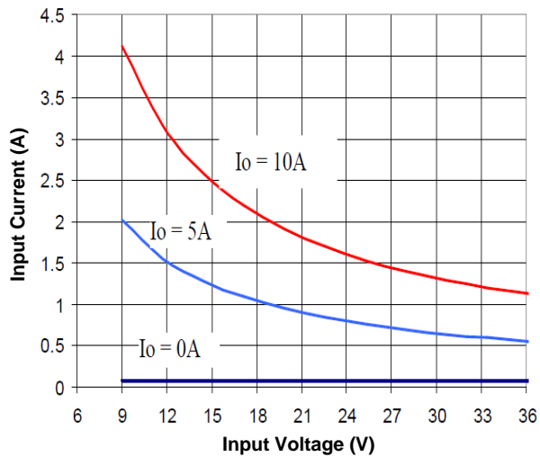
Figure 2. Input Characteristic (5V output)
