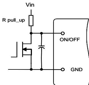
Figure12. Circuit for Logic Control
