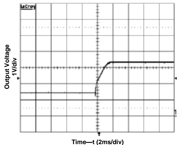
Figure 3. Start-Up with Prebias (Input voltage 24V, Output current 0A, Output voltage 3.3V, Prebias 1.8V)
