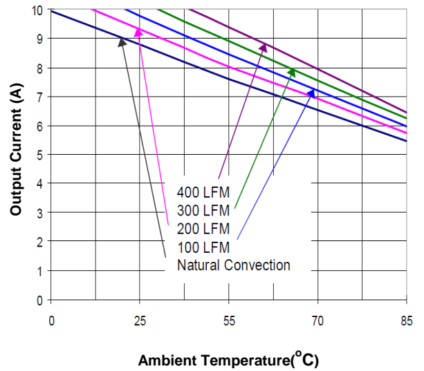
Figure 11(b) . Current Derating Curve for 5V Output ( V_{in} = 24V open frame)
