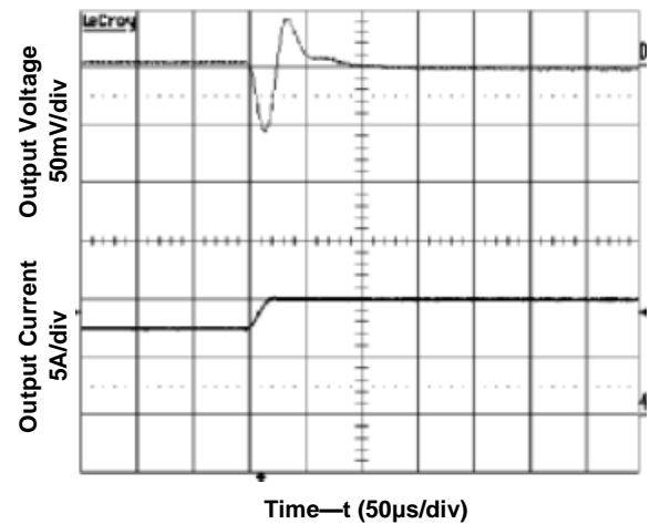
Figure 9. Transient Load Response Input voltage 24/3.3V, Output current 7.5A->10A, Slew rate 0.1A/µs
