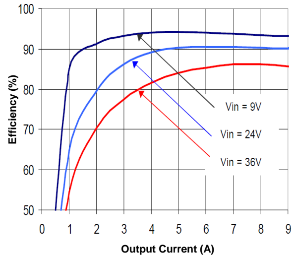
Figure 1(b). Efficiency vs. Load Current (25°C, 5V)
