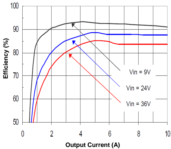
Figure 1(a). Efficiency vs. Load Current (25°C, 3.3V)
