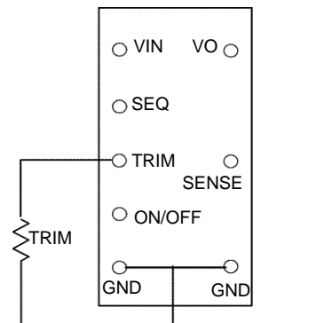
Figure 13. Circuit to Trim Output Voltage.
