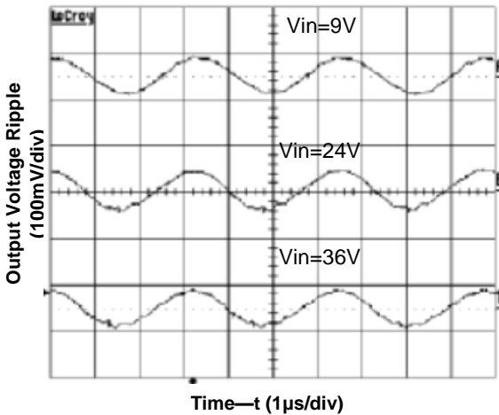
Figure 6. Output Ripple Voltage at 5V, 9A Output
