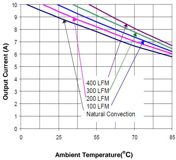
Figure 11(a) . Current Derating Curve for 3.3V Output ( V_{in} = 12V open frame)
