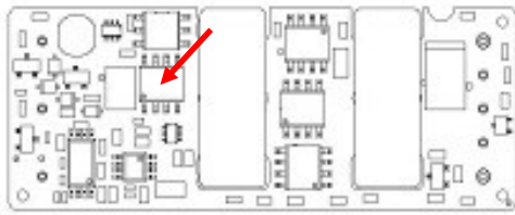
Figure 15. Temperature Monitoring Locations
