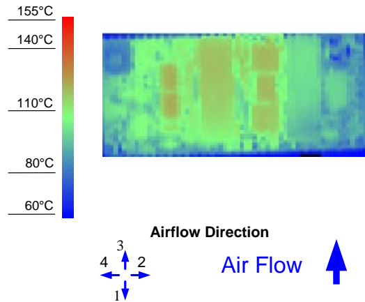
Figure 8. Thermal Image for Airflow Direction 3 (23.5A output, 55°C ambient, 200 LFM, typical Vin, open frame, unit soldered onto a fixture board)
