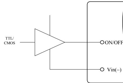
Figure 12. Direct Logic Drive
