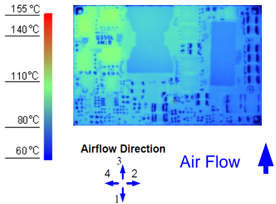
Figure 9. Thermal Image for Airflow Direction 3 (35.5A output, 55°C ambient, 200 LFM, typical Vin, open frame, unit soldered onto a fixture board)
