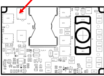
Figure 15. Temperature Monitoring Locations
