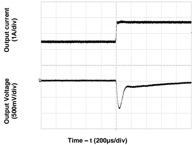
Figure 8. Transient Load Response (typical V_{in} , load current steps from 50% to 75% at a slew rate 0.1A/µs)
