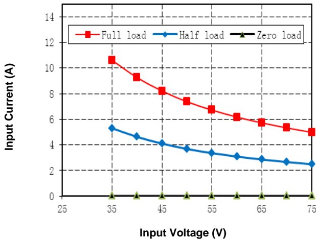
Input Voltage (V) Figure 3. Input Characteristics (25°C)
