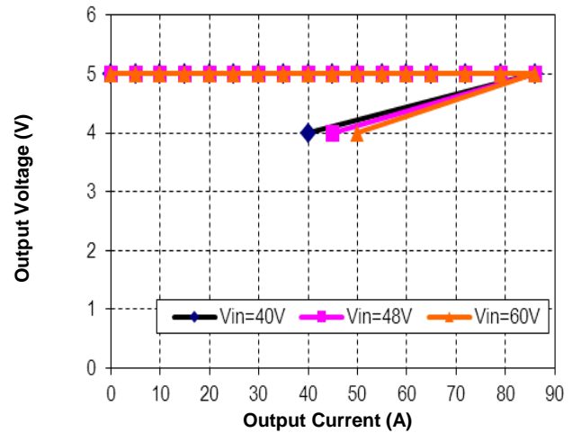
Output Current (A) Figure 4. Output Characteristics (non-parallel)
