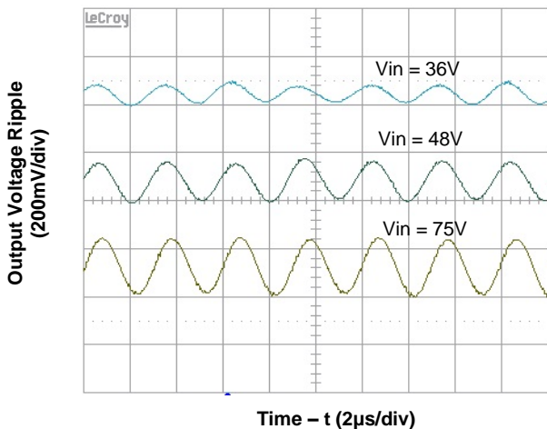
Time - t (2µs/div) Figure 5. Output Ripple Voltage at Full Load
