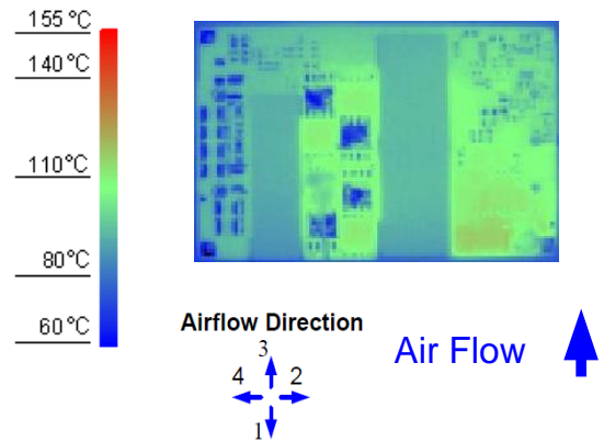
Figure 10. Thermal Image for Airflow Direction 3 (48A output, 75°C ambient, 200 LFM, typical Vin, open frame, soldered interface)
