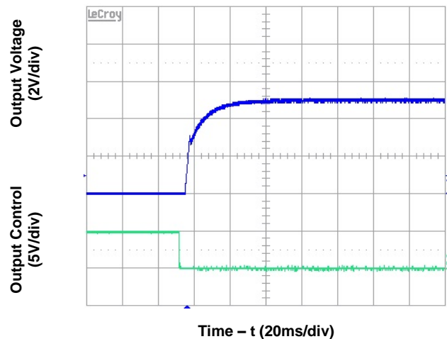
Time - t (20ms/div) Figure 6. Start-Up from Enable Control (typical Vin, zero load, no external Cap.)
