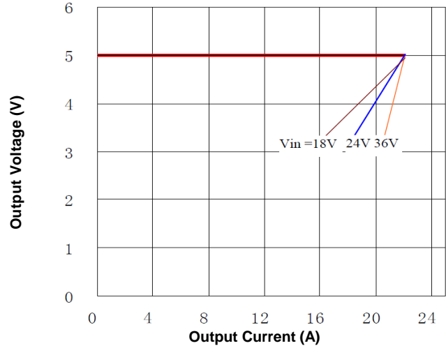
Figure 8. Output Characteristic (25°C)
