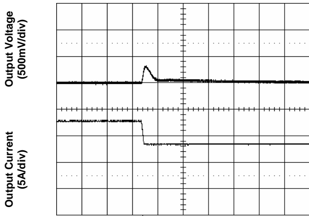
Figure 9. Transient Load Response (typical V_{in} , load current steps from 75% to 50% at a slew rate 0.1A/ \mu s)
