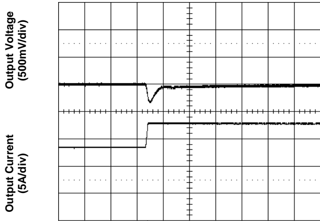
Figure 10. Transient Load Response (typical V_{in} , load current steps from 50% to 75% at a slew rate 0.1A/ \mu s)
