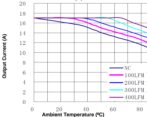
Figure 11. Derating Curve for Airflow Direction 3 (Ref. Figure 12 for Airflow Direction; typical V_{in} ; open frame, unit soldered into fixture board)
