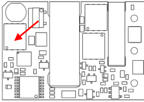
Figure 19. Temperature Monitoring Locations
