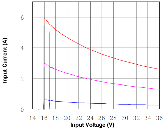
Figure 7. Input Characteristic (25°C)
