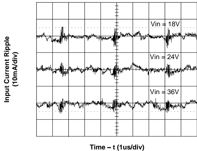
Figure 4. Input Reflected Ripple Current at Full Load
