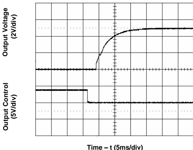
Figure 5. Start-Up from Enable Control (typical Input voltage and full load)
