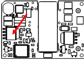
Figure 15. Temperature Monitoring Locations
