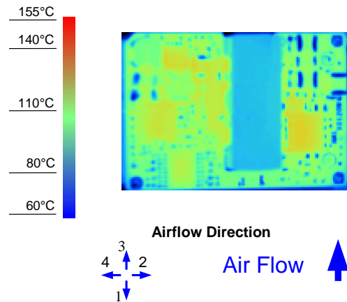
Figure 8. Thermal Image for Airflow Direction 3 (5A output, 55°C ambient, nature convection, typical Vin, open frame, unit soldered onto a fixture board)
